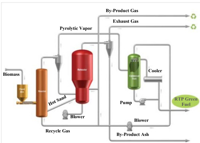
RTP Process Flow Diagram
